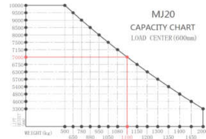
Capacity Chart-MJ20
